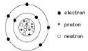
One atom of nitrogen
